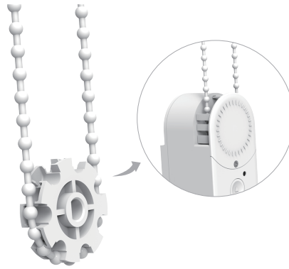
Bead diameter \Phi 4 \sim 4.5\text{mm} With spacing 6 \sim 6.5\text{mm}
