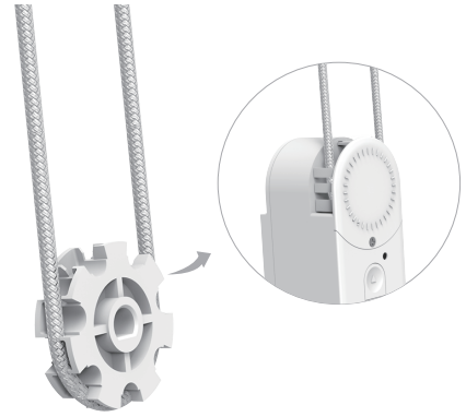
Cord diameter: \Phi 3.5 \sim 3.8\text{mm}
